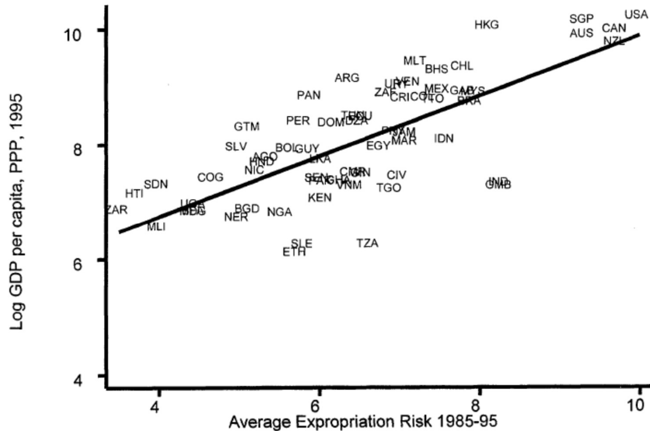
FIGURE 2. OLS RELATIONSHIP BETWEEN EXPROPRIATION RISK AND INCOME
